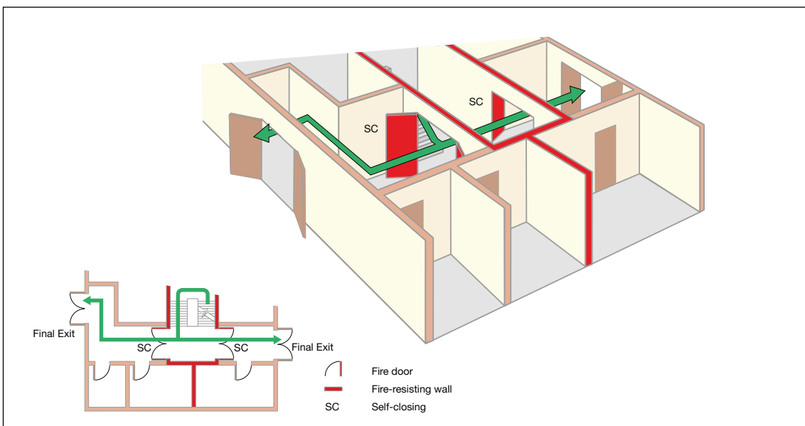
Figure 34: Example of two escape routes from a stairway to a final exits
