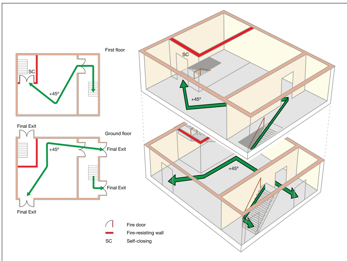
Figure 42: Two-storey, lower risk (e.g. church hall)
