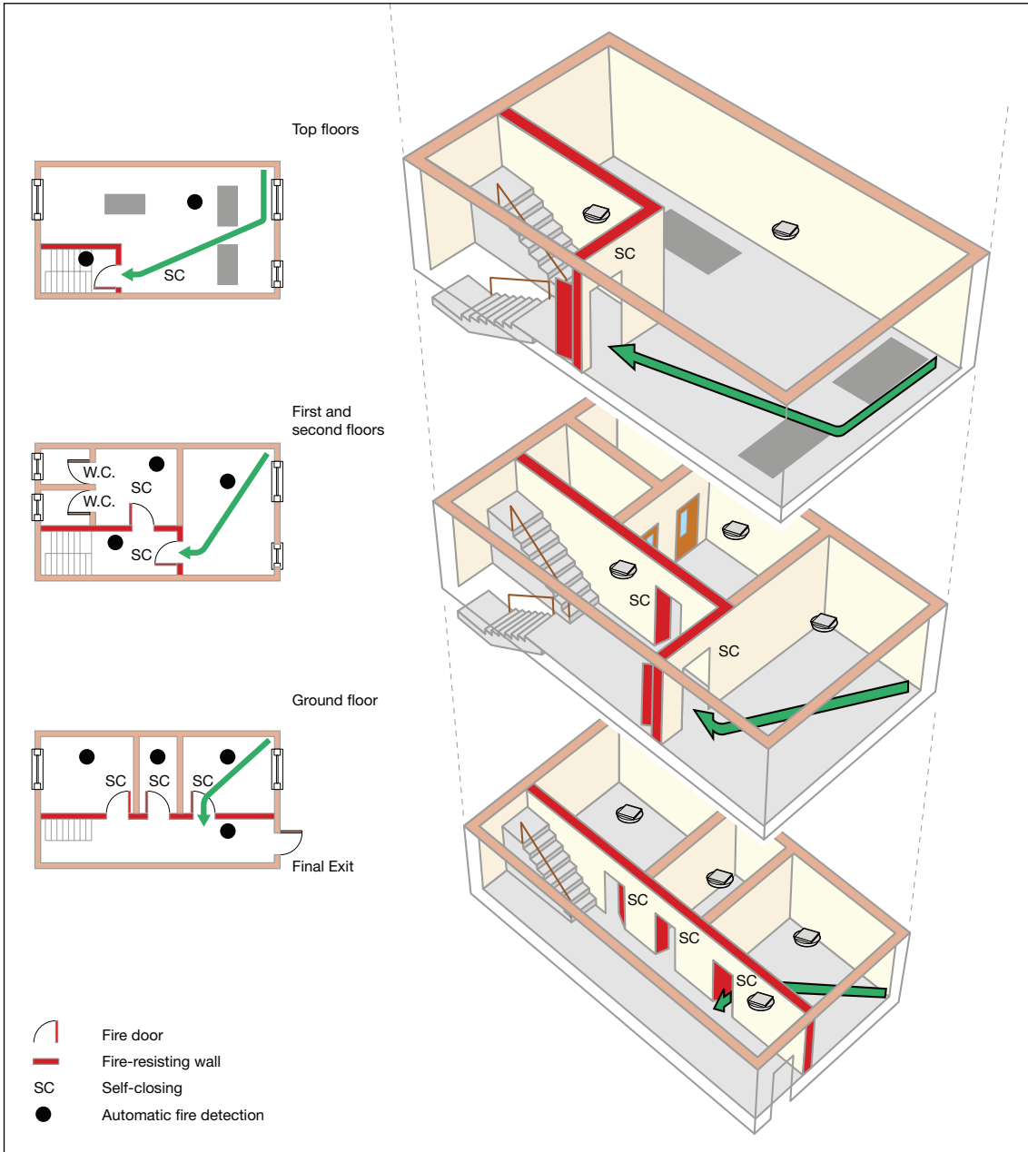
Figure 50: Four-storey, ground and up to three upper floors – protected with automatic fire detection
