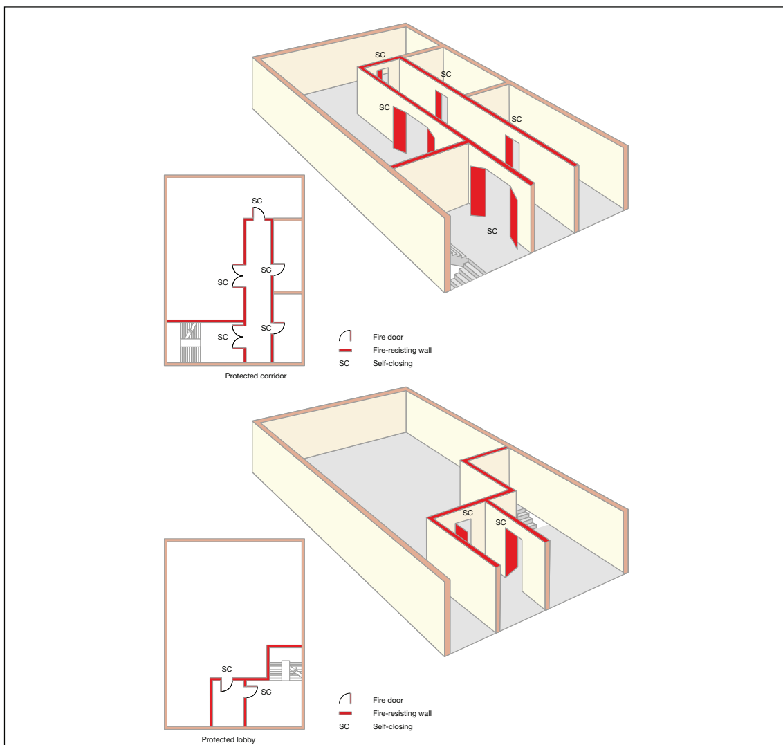
Figure 32: Examples of a stairway with protected lobby/corridor approach
