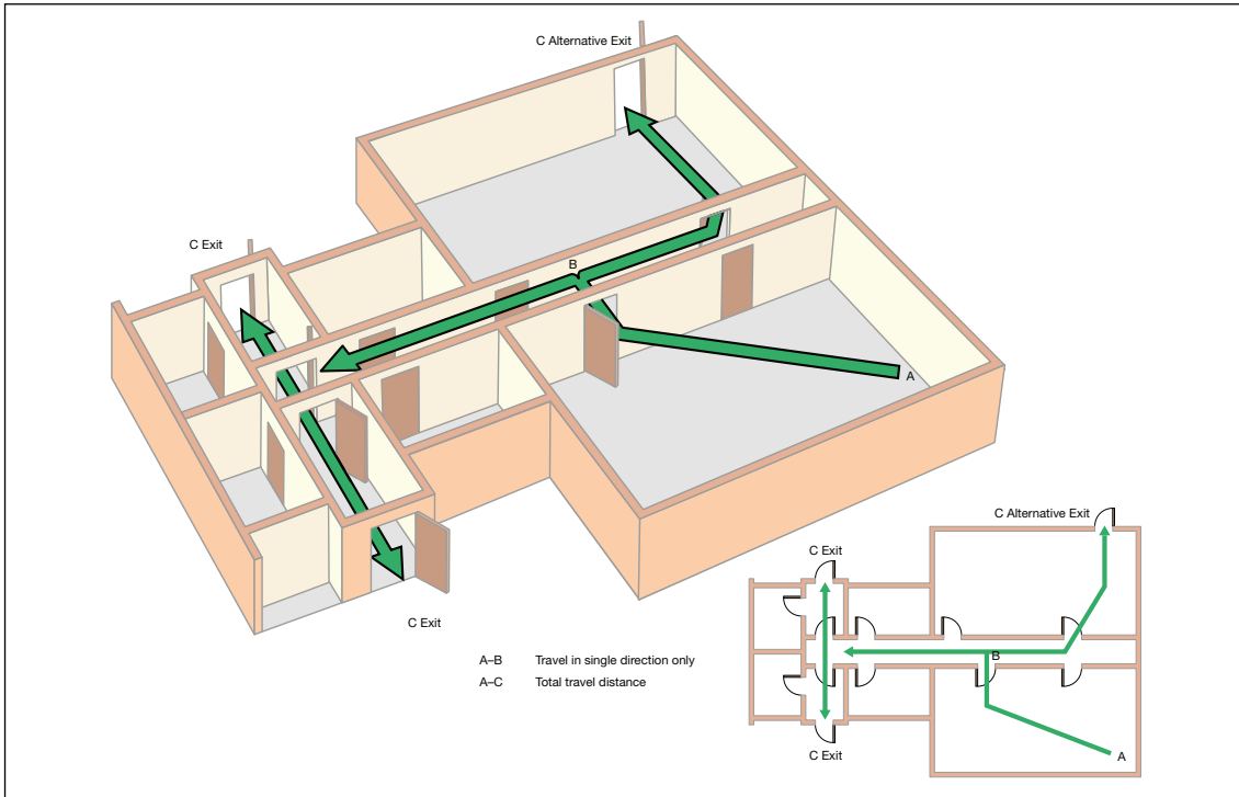
Figure 29: Dead-end condition provided with an alternative exit
