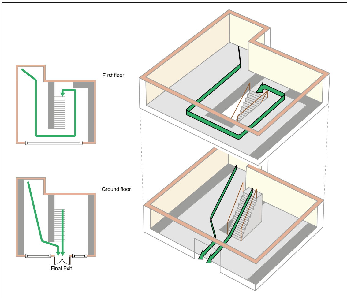
Figure 45: Two-storey, ground and one upper floor with a single stairway
