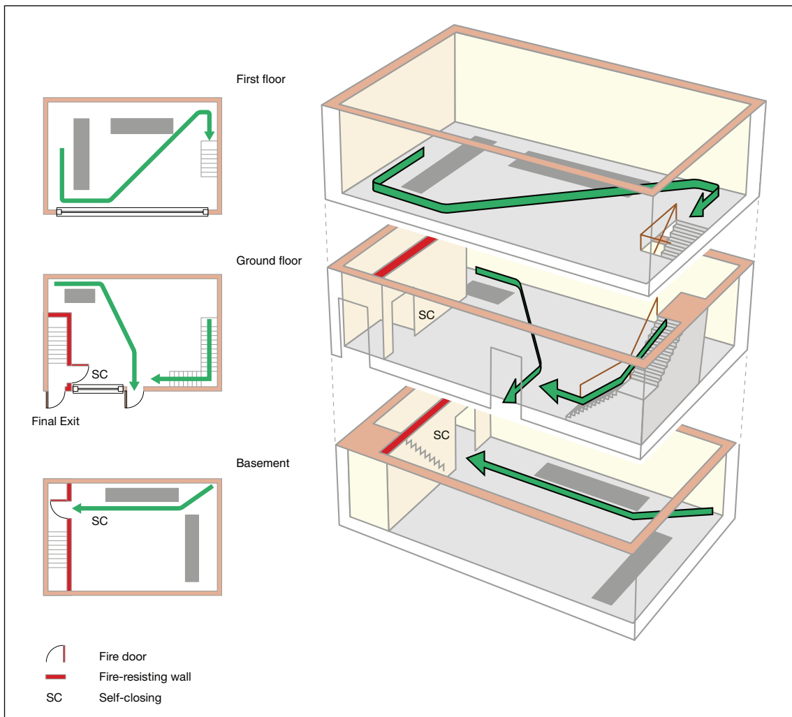
Figure 47: Three-storey, small basement, ground and one upper floor
