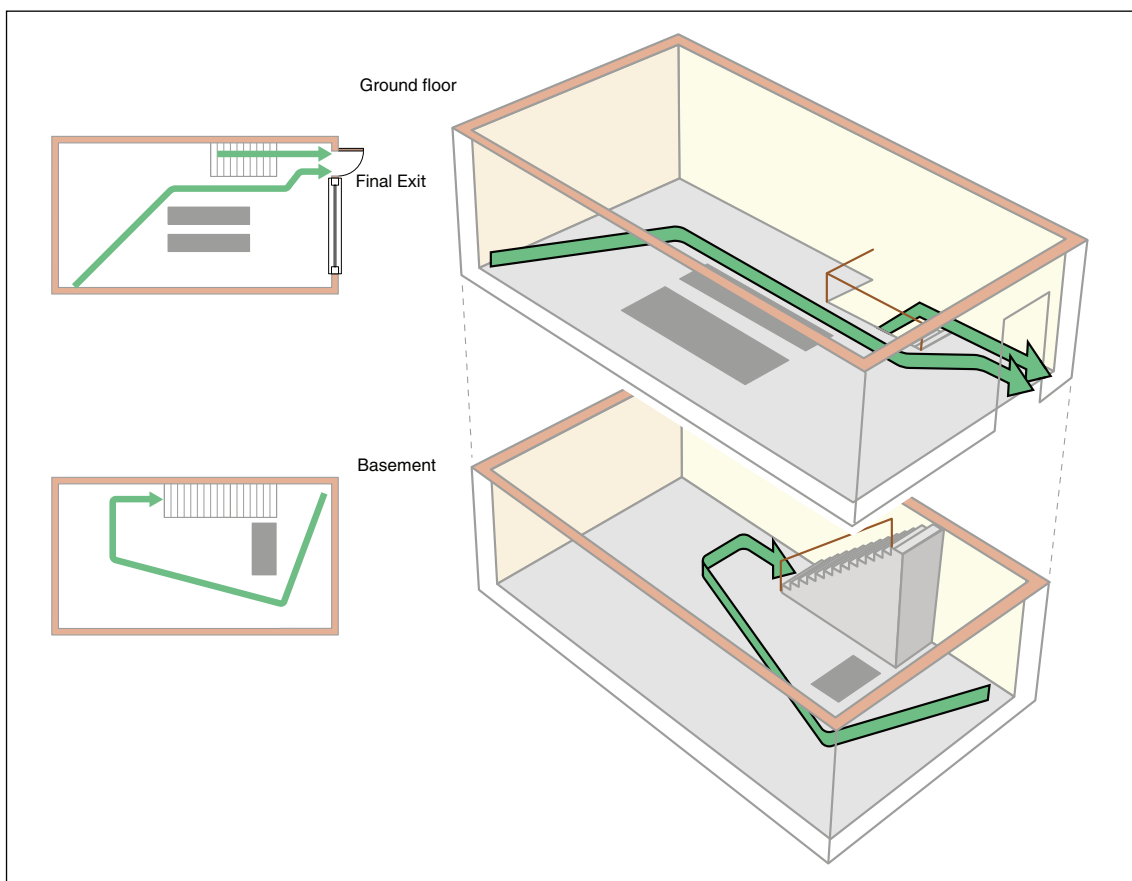
Figure 46: Two-storey, basement and ground floor with a single stairway
