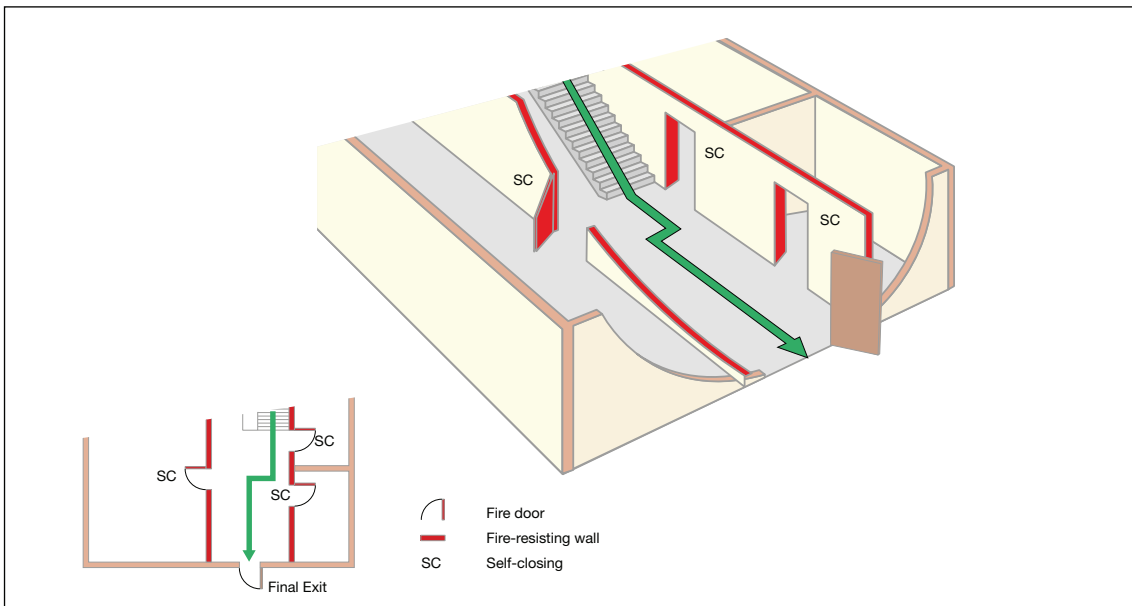
Figure 33: Example of a protected route from a stairway to a final exit
