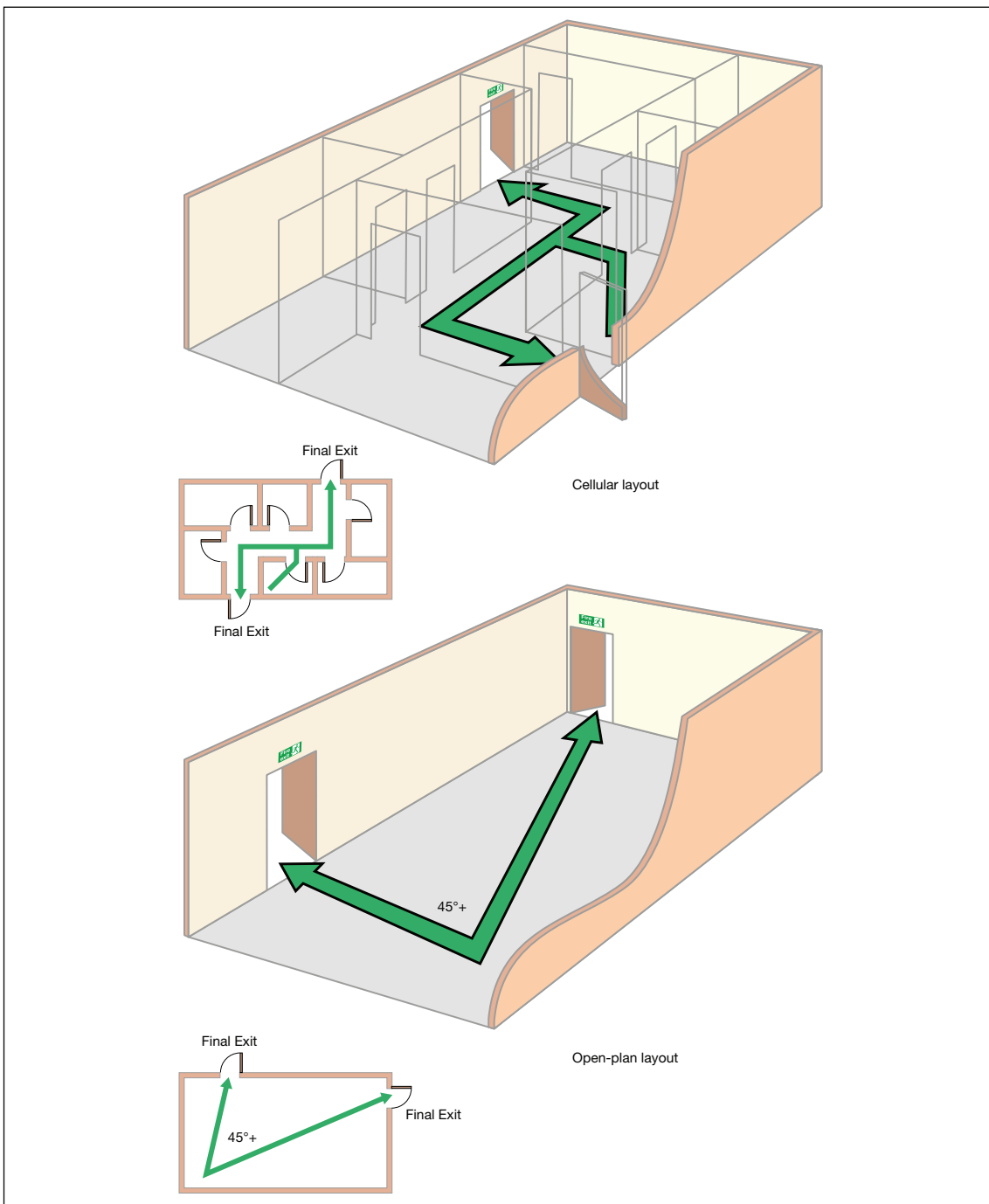
Figure 41: Ground floor with more than one exit
