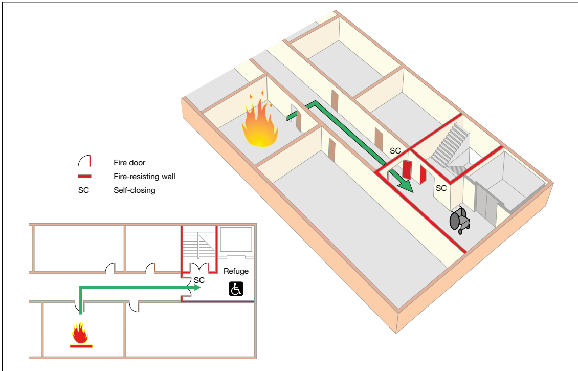
Figure 20: An example of a refuge
