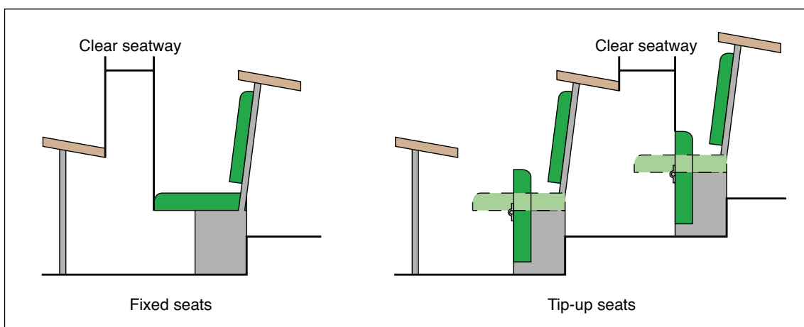
Figure 19: Clear space between seating
