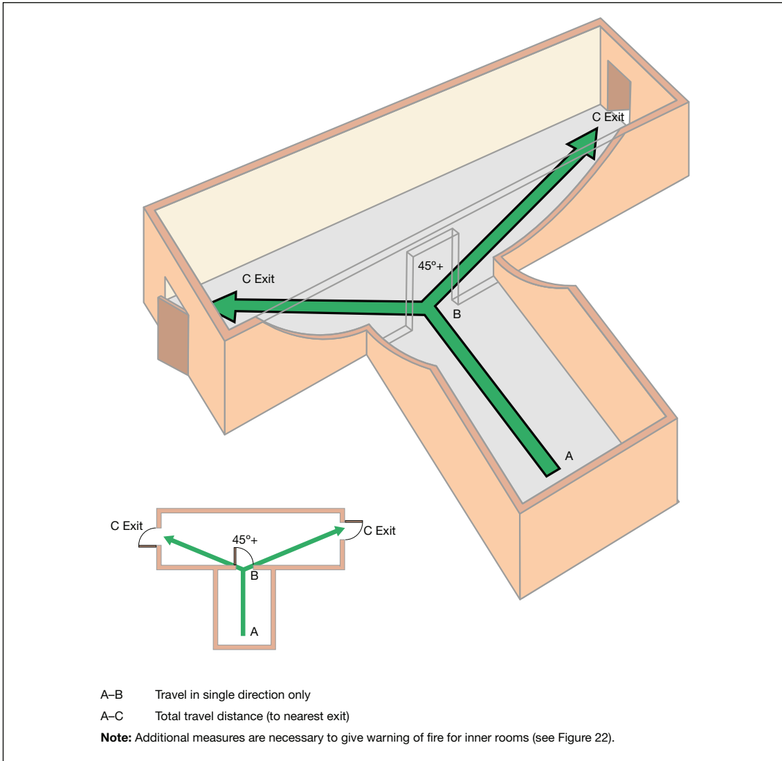
Figure 26: Measuring travel distance from initial dead end (inner room)
