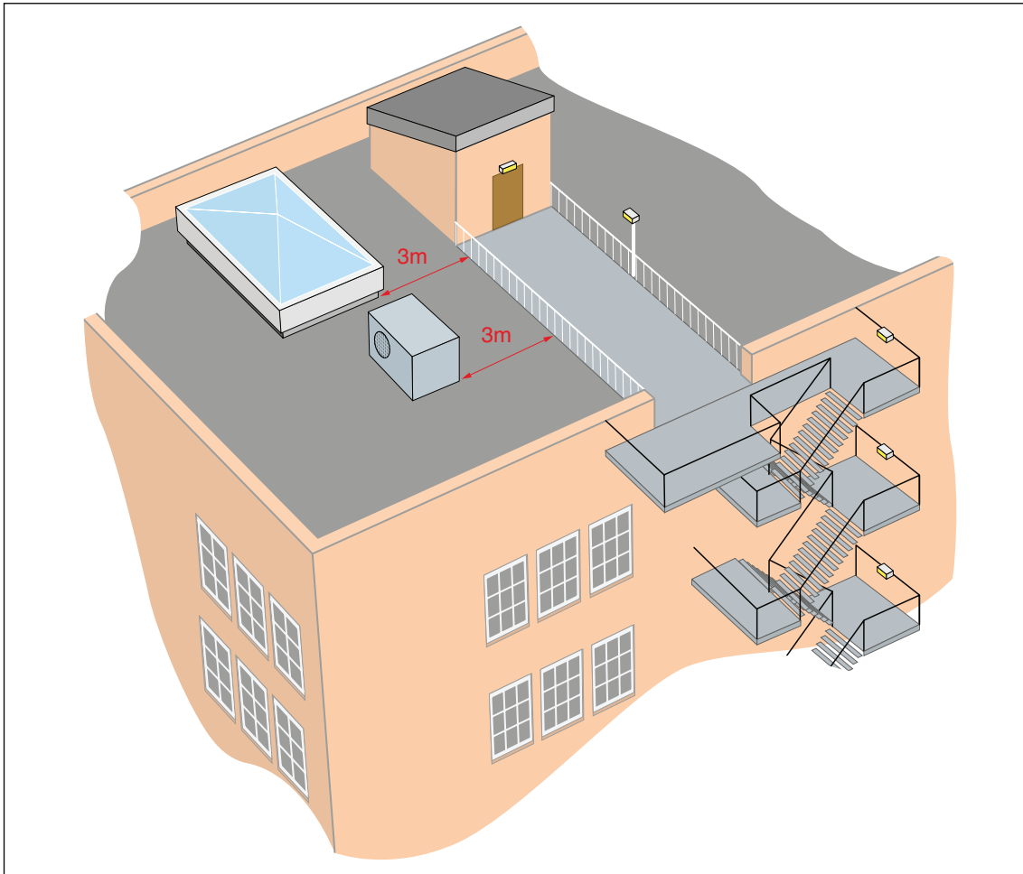
Figure 38: An escape route across a roof
