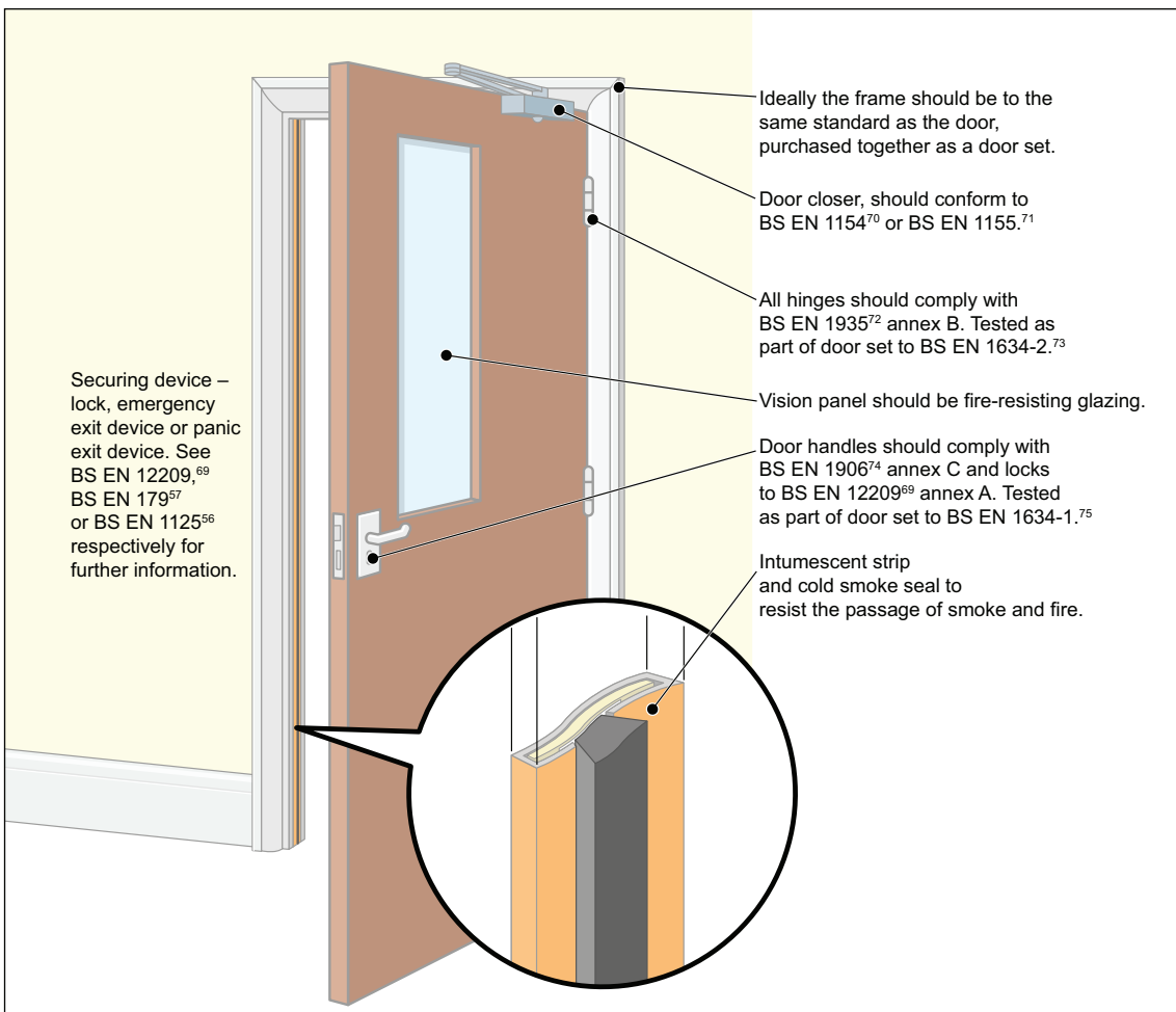
Figure 61: A fire-resisting and smoke stopping door
