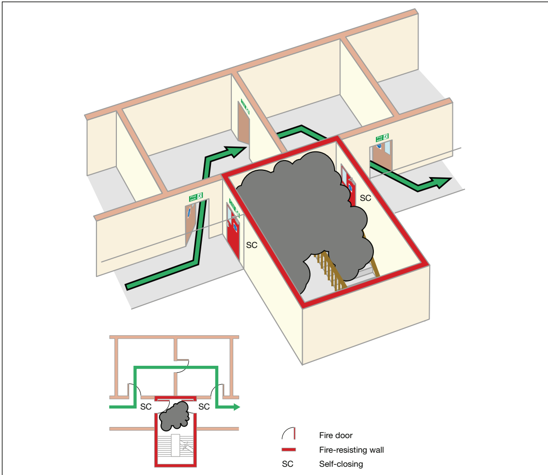
Figure 36: A stairway bypass route
