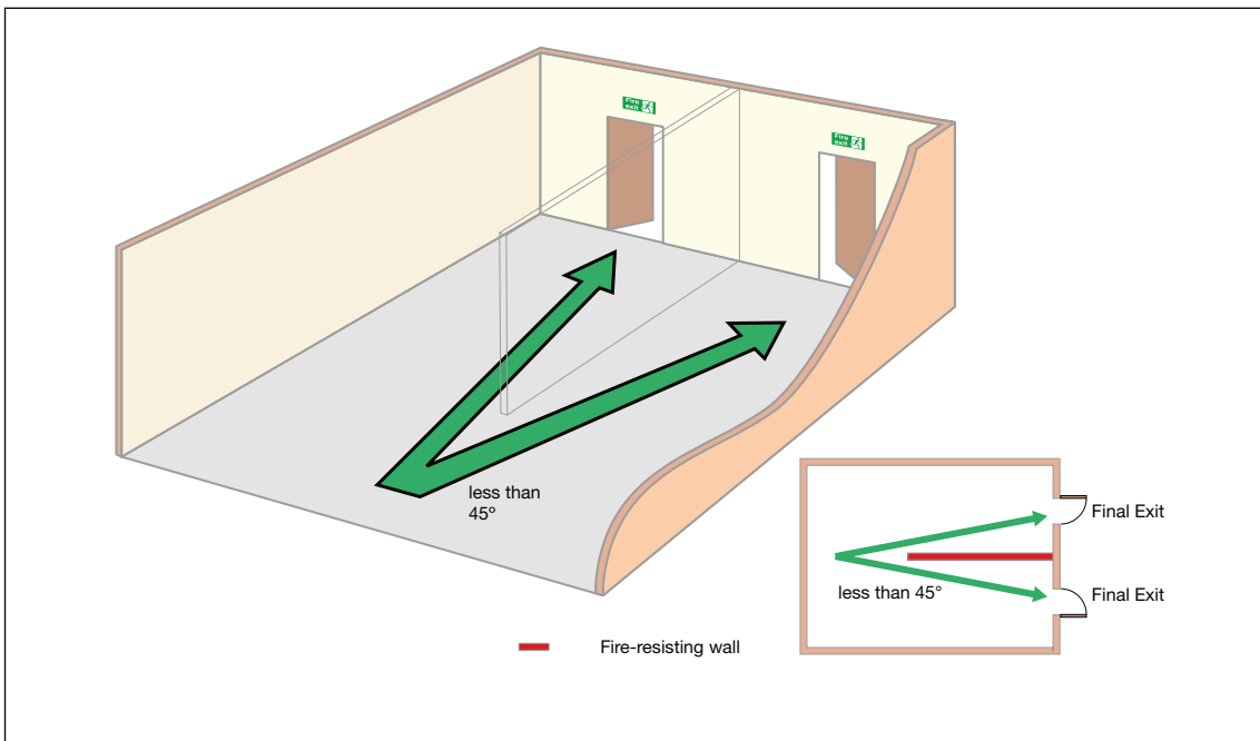
Figure 24: Alternative exits (separated by fire-resisting construction)
