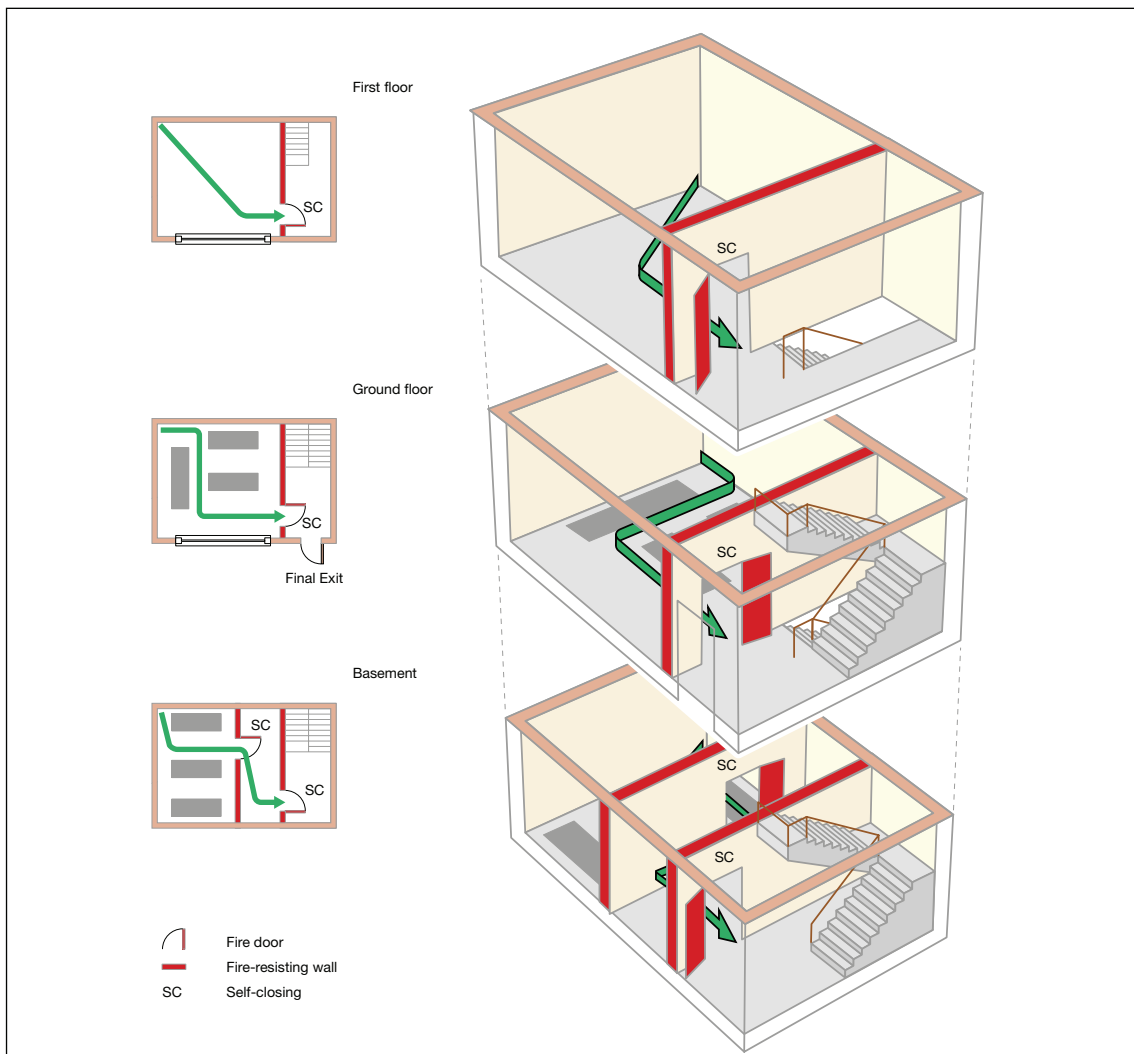
Figure 48: Three-storey, basement, ground and one upper floor
