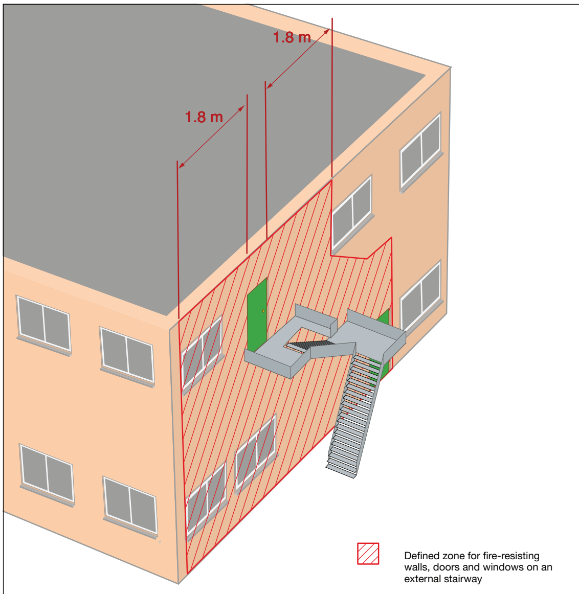
Figure 37: Protection to an external stairway
