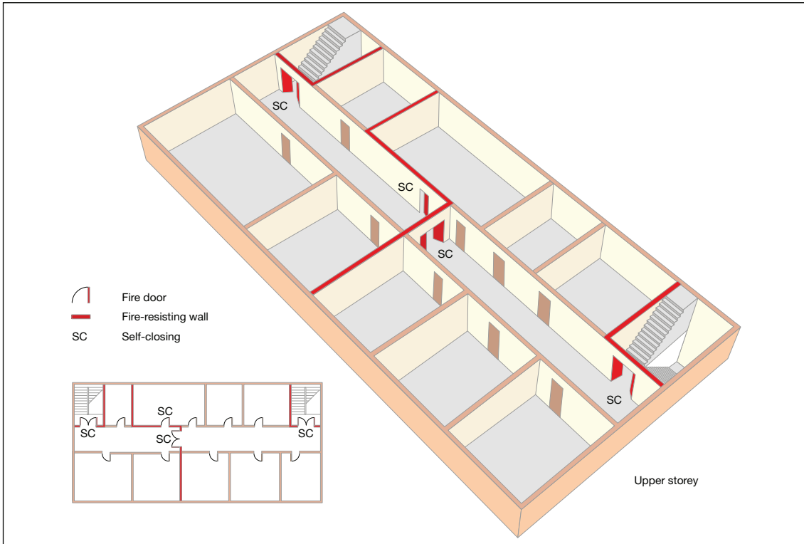
Figure 31: Subdivision of corridor between two stairways or exits
