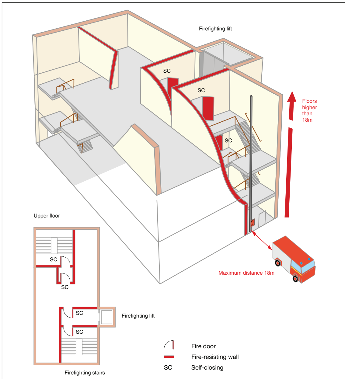
Figure 44: Tall building with a firefighting shaft
