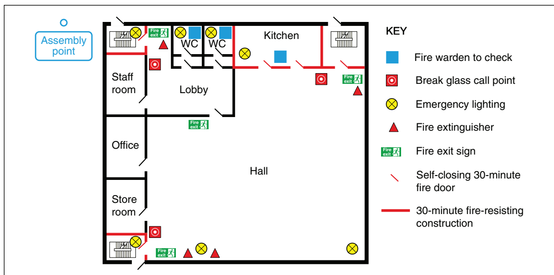
Figure 12: Example of a line drawing general fire safety precautions
