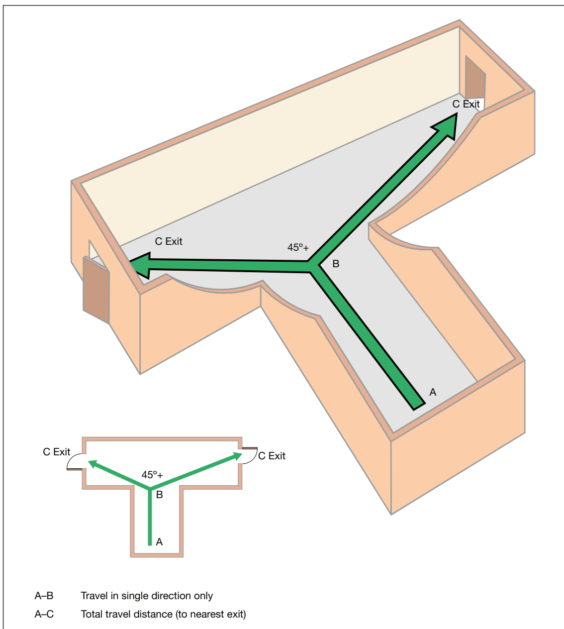
Figure 25: Measuring travel distance from initial dead end (open plan)
