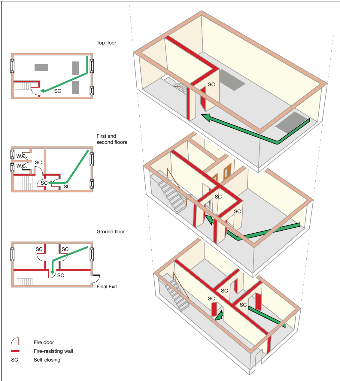
Figure 49: Four-storey, ground and up to three upper floors – protected by lobbies/corridors
